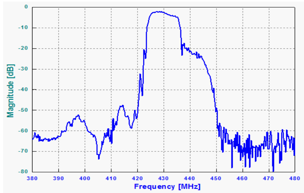
Frequency Response
